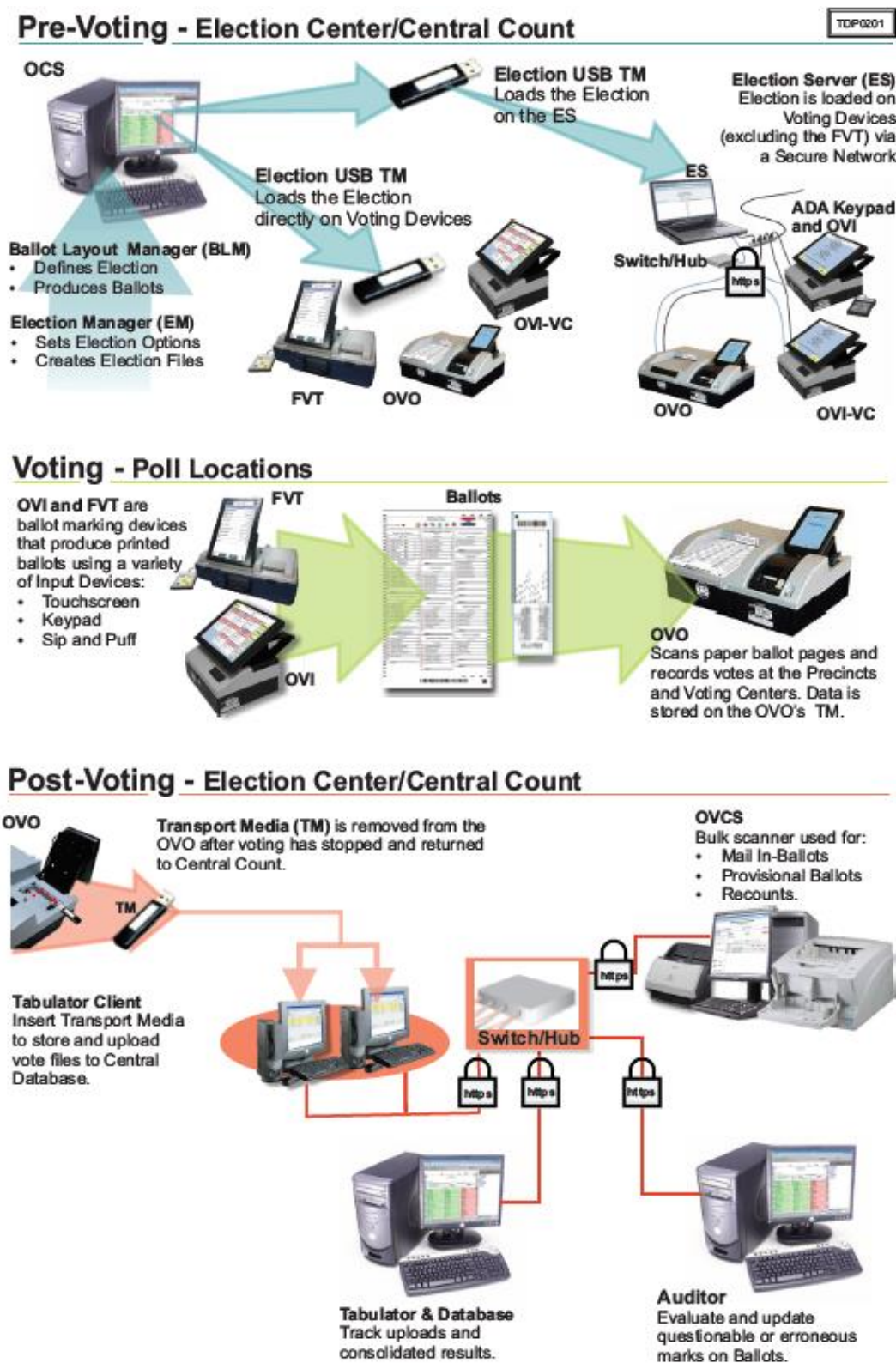
Figure 1-5. OVS 2.0 System Components Overview
